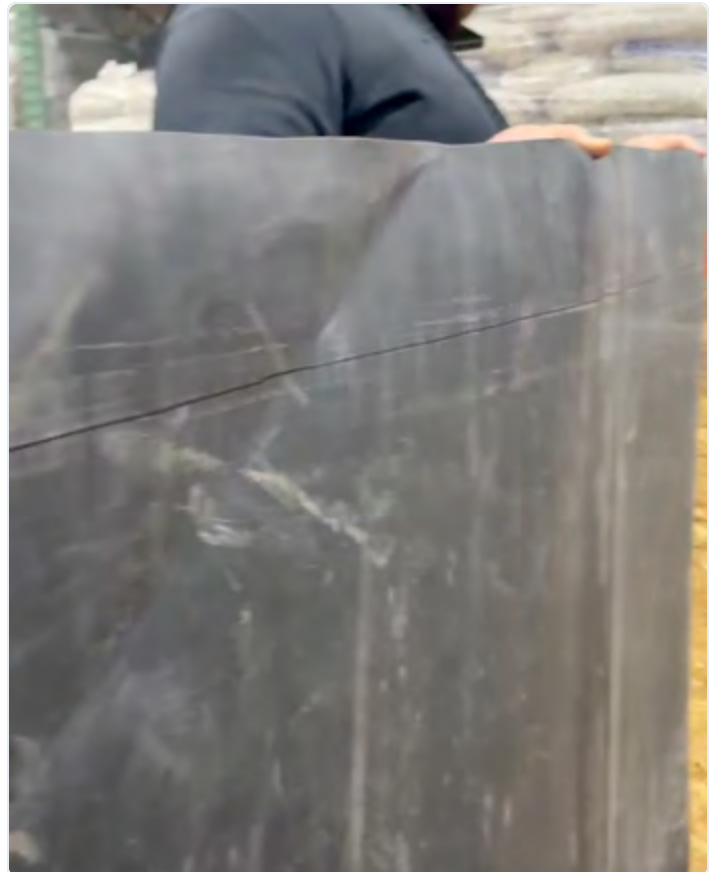
FIG VW.2 Dry-fit with the top overlap projecting above the wall edge. The sharpie line along the wall top becomes the alignment reference for glue-up.
